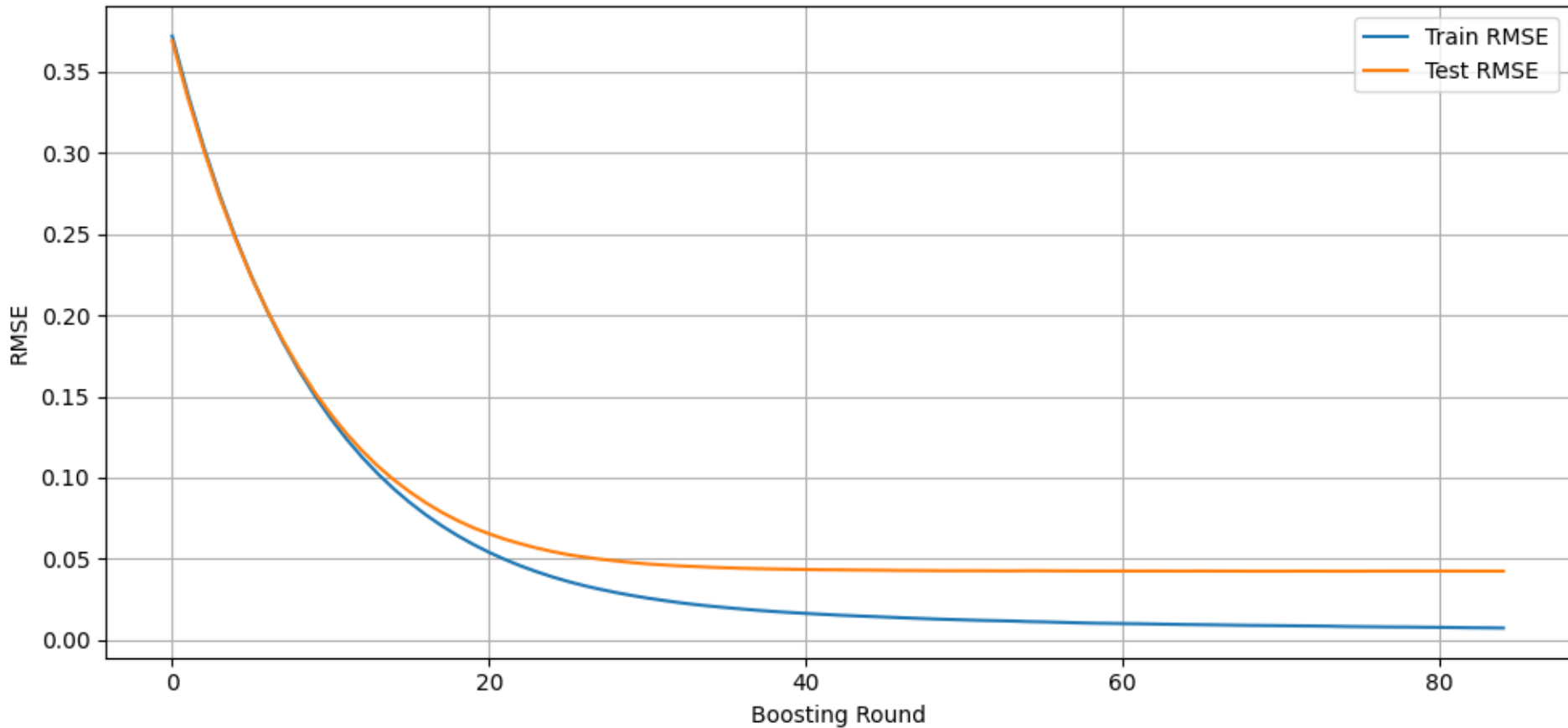
XGBoost Training vs Test RMSE
