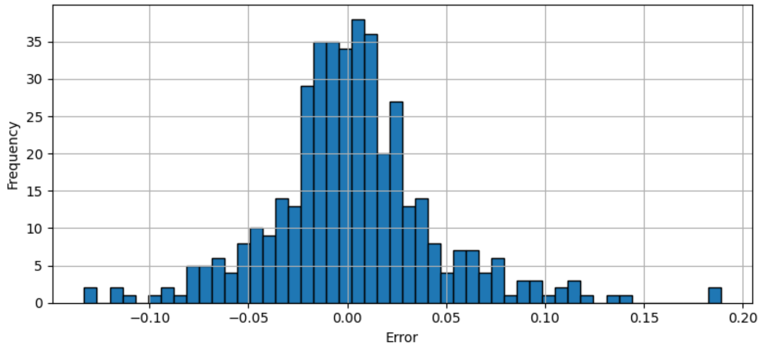
Prediction Residuals
